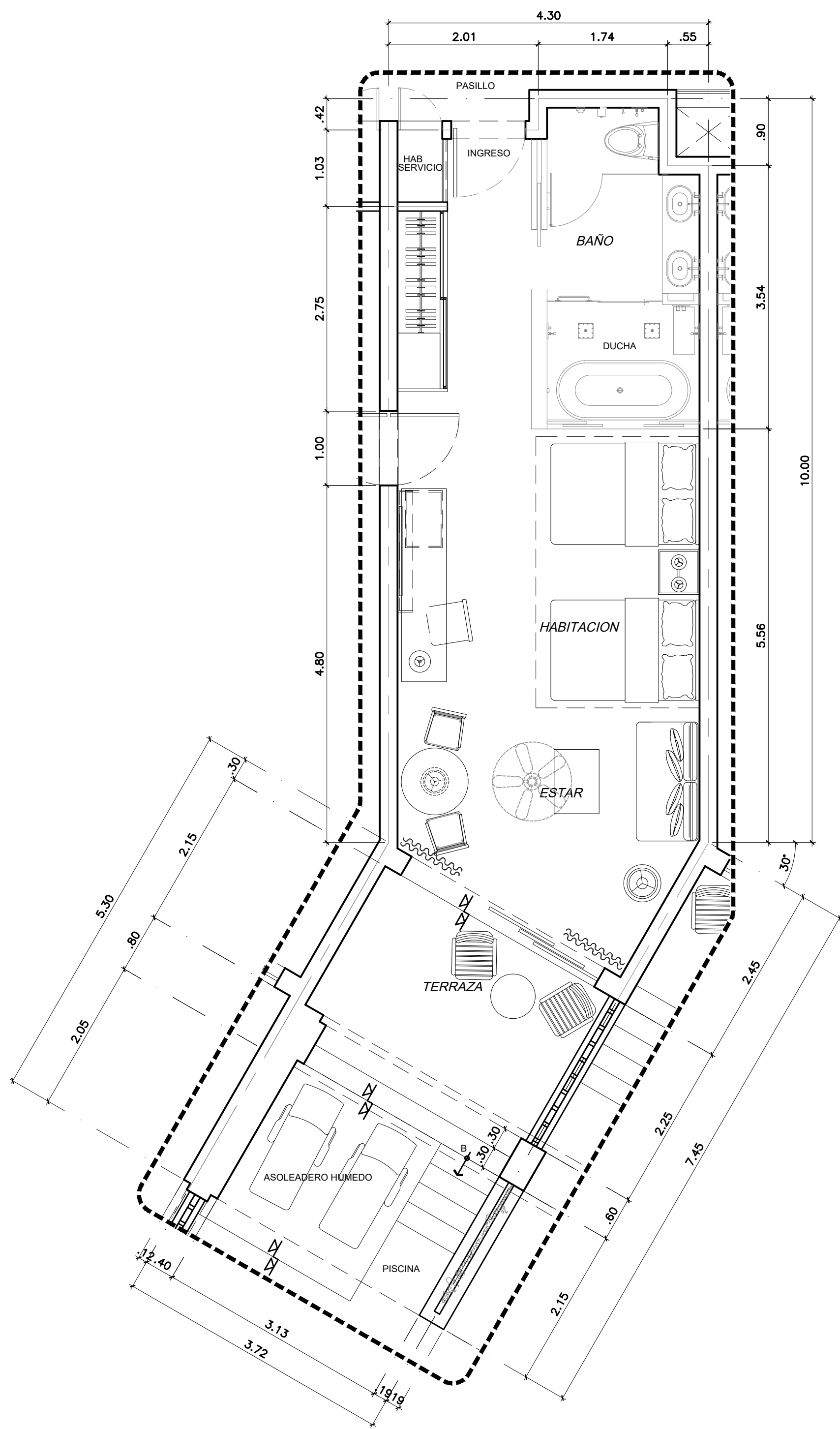
HABITACION JUNIOR SUITE DIAGONAL PREFERRED PB "A" INTERCOM ESC. 1:50 METROS
